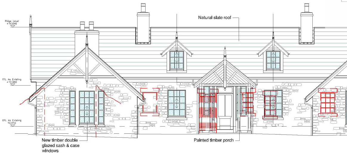
North East Elevation 1:100
